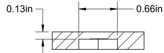
SECTION C-C SCALE 1 : 1
